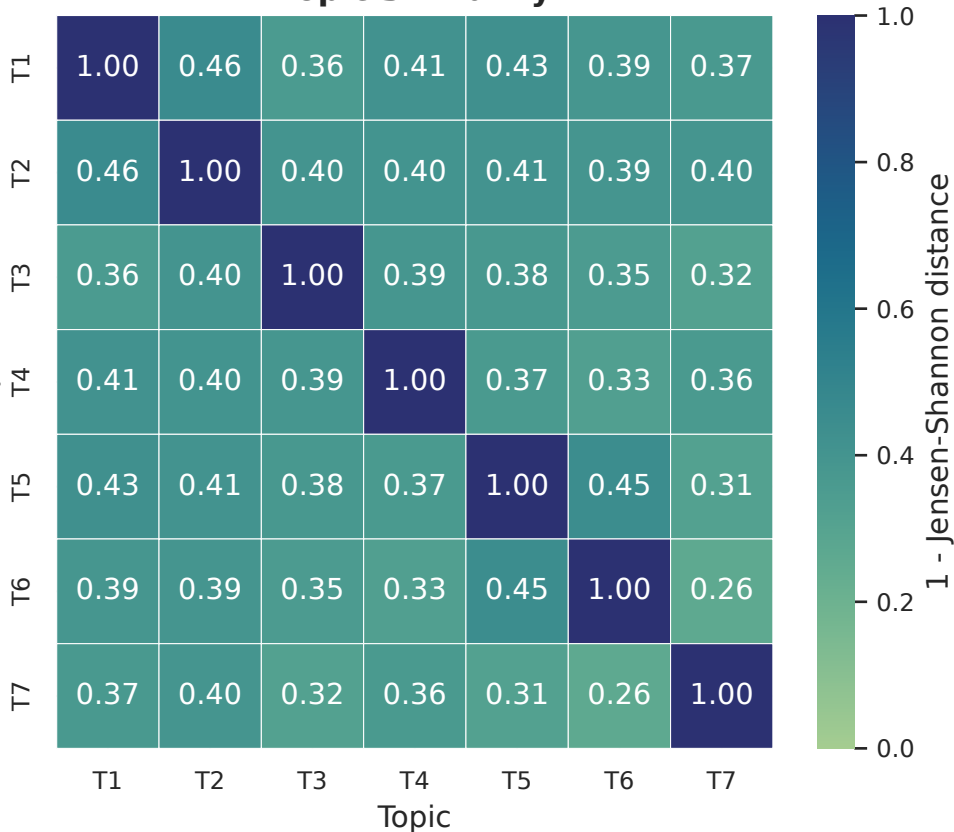
Topic similarity
