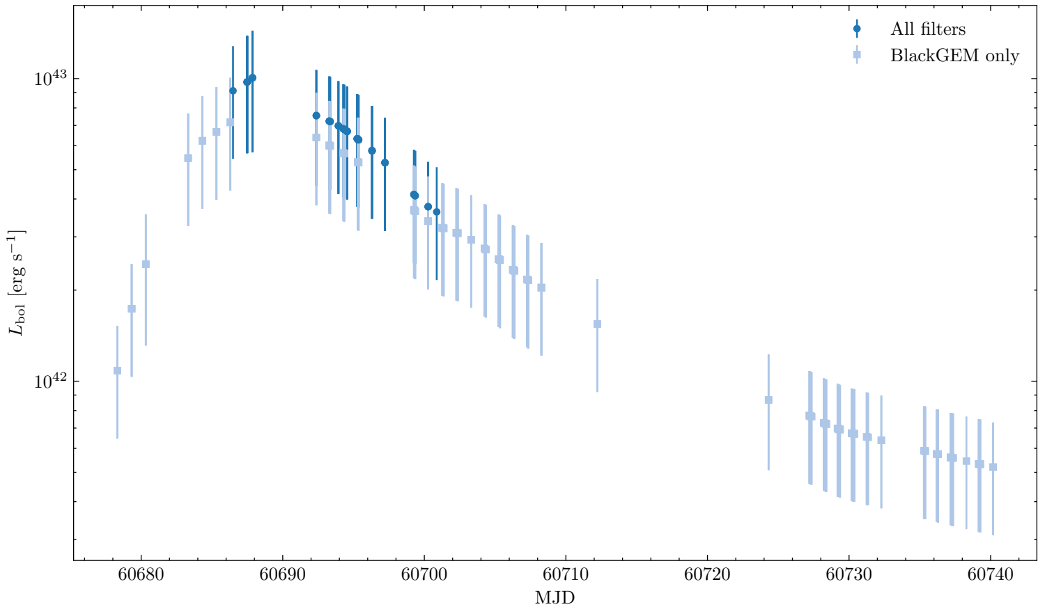
Pseudobolometric light curve for SN2025cy
