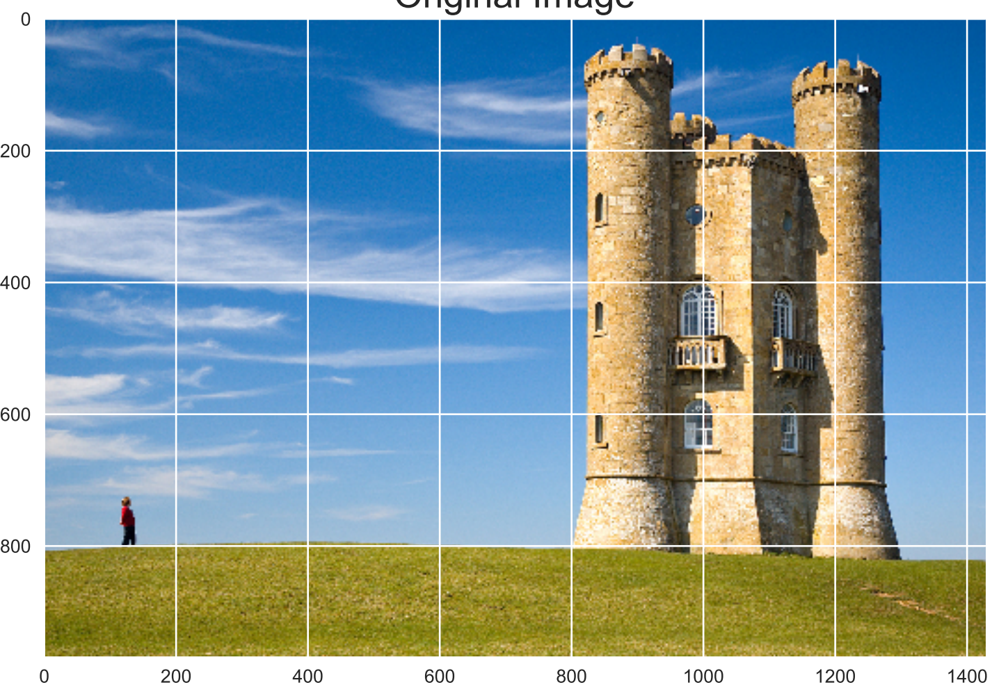
Original Image
