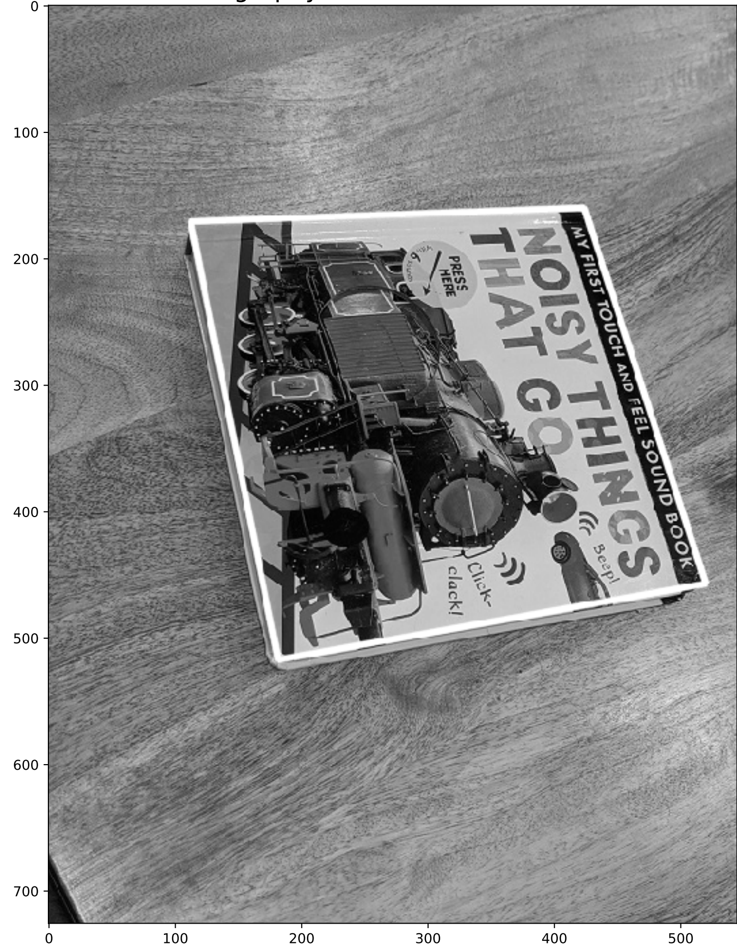
Homography Estimated With RANSAC
