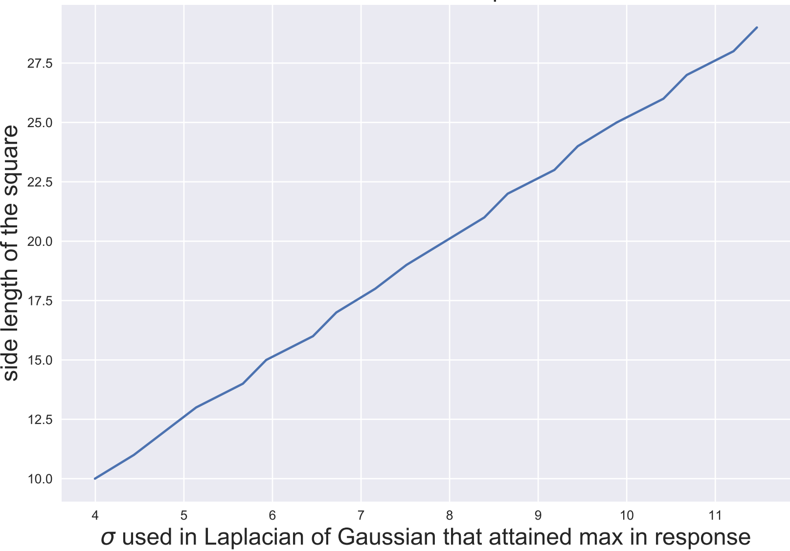
relationship between response maximizer ( \sigma used in LoG), and the size of square
