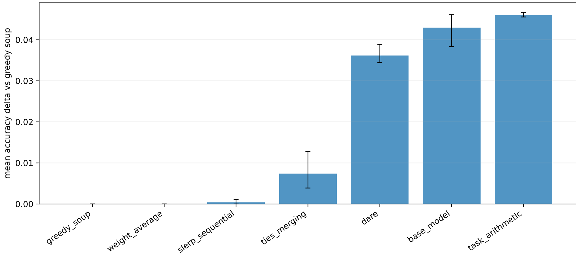
Same-base task-vector methods
