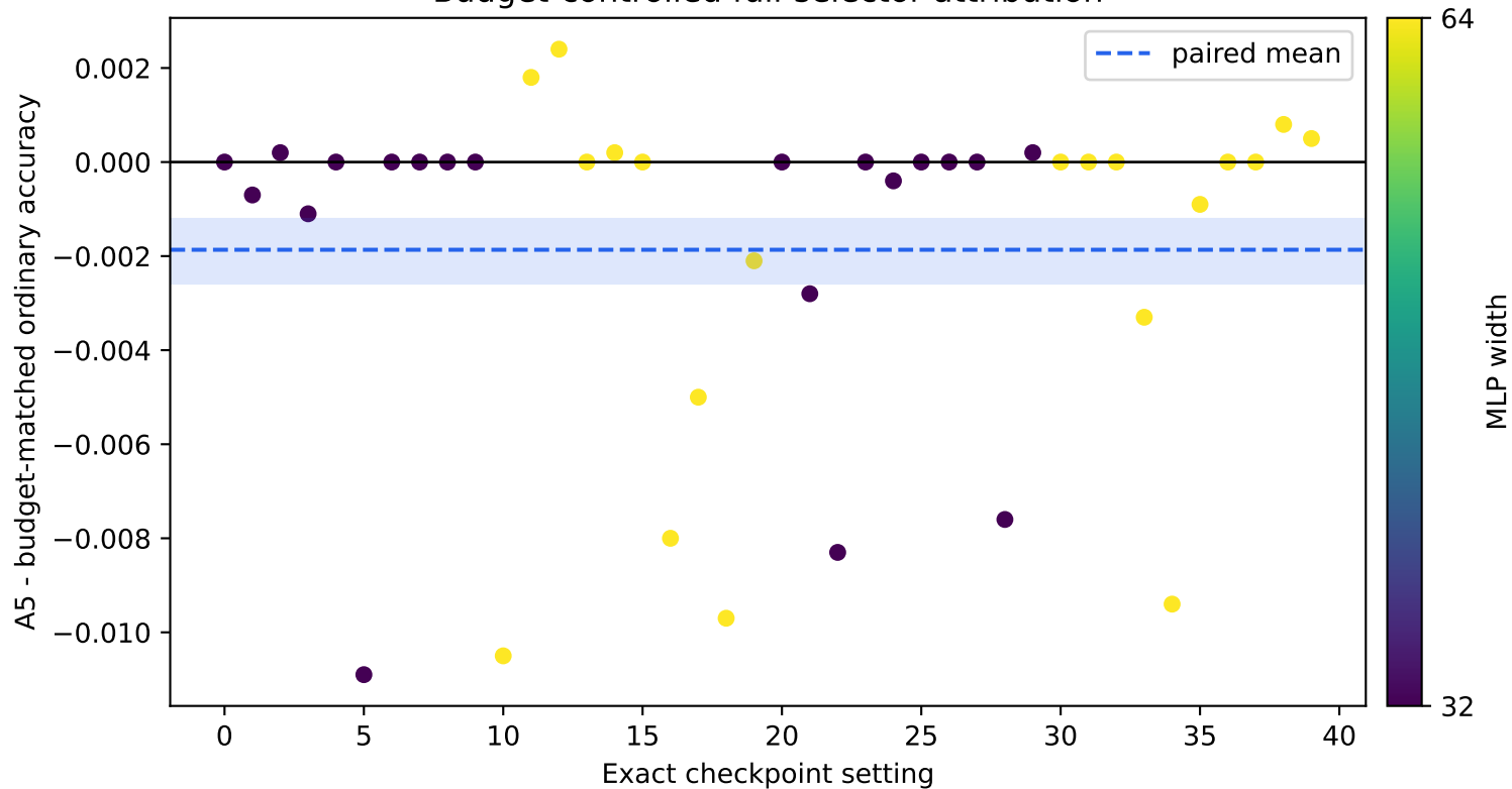
Budget-controlled full-selector attribution
