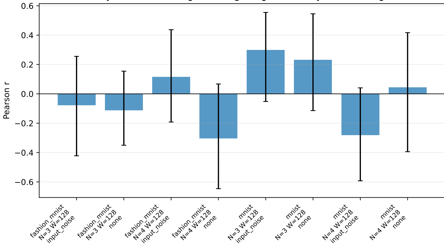
Cycle score vs weight-average degradation by fixed setting
