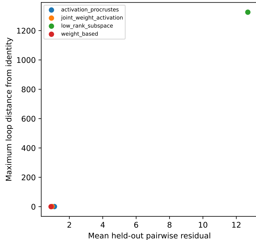
Pairwise fit does not equal loop consistency
