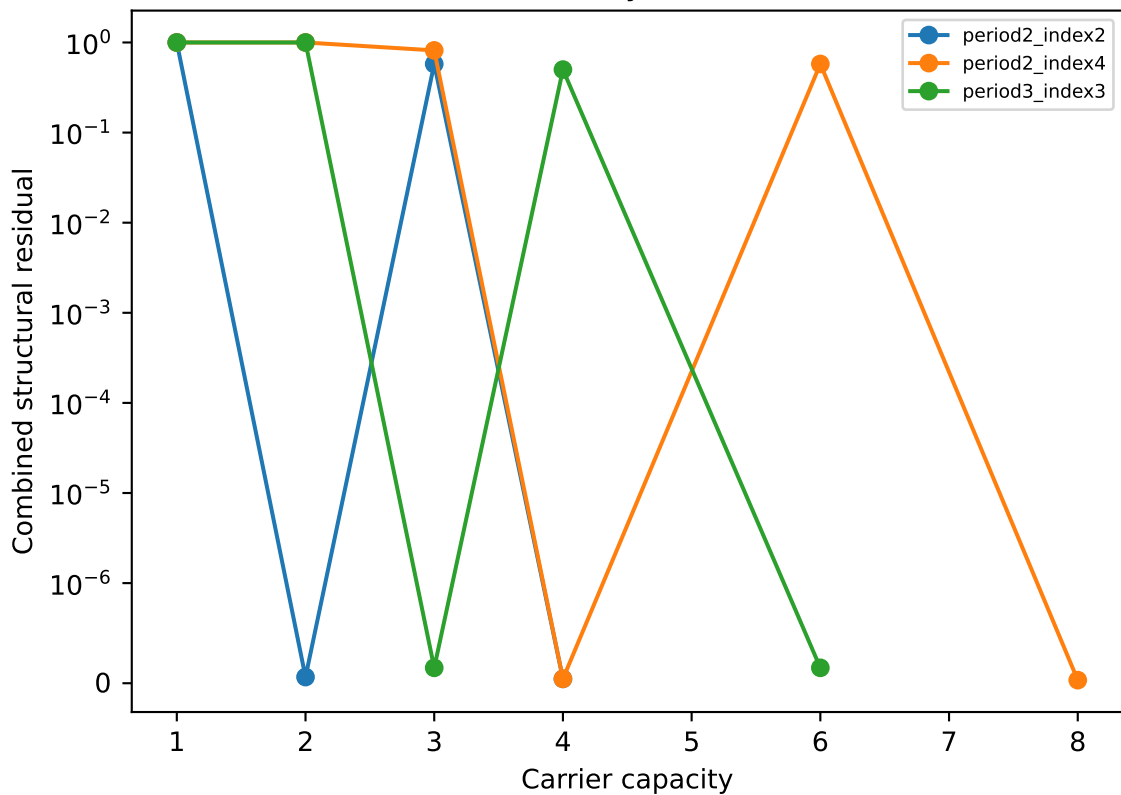
Index divisibility and structure
