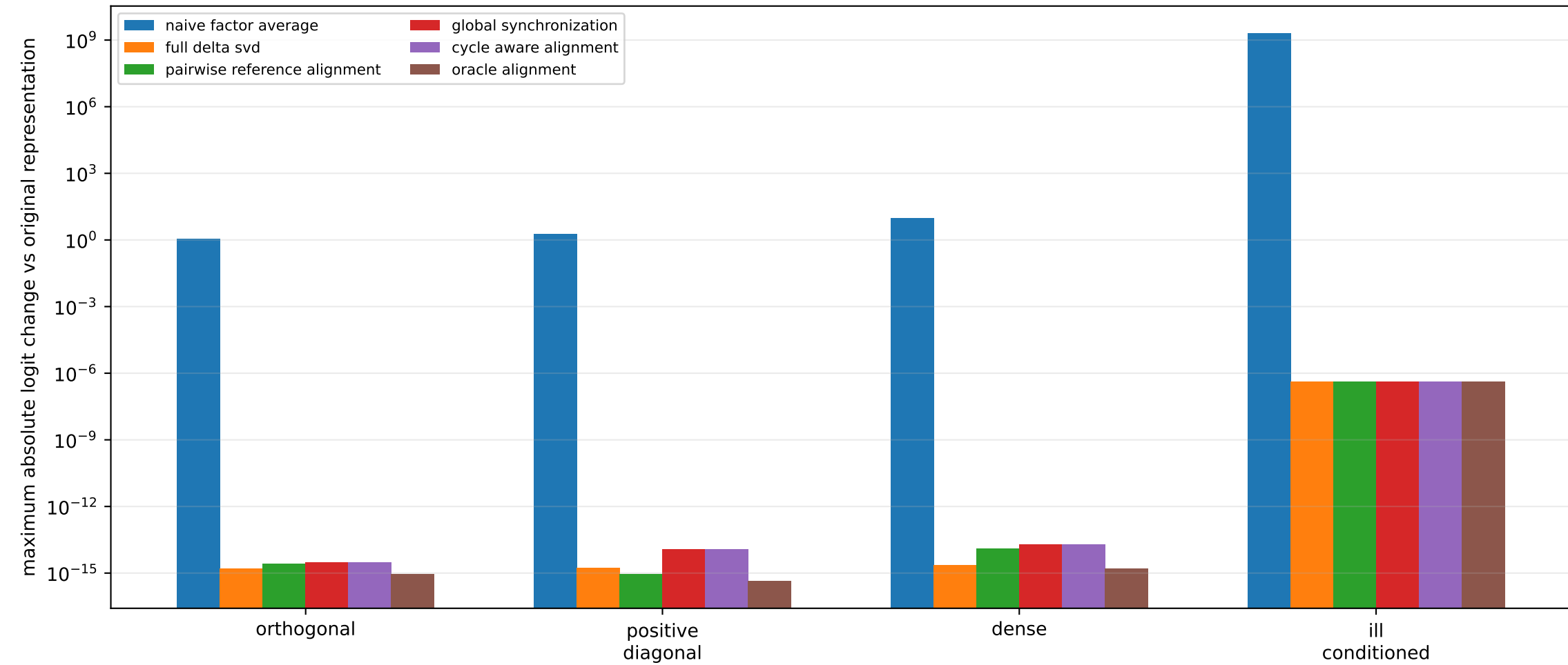
One fixed adapter group across dependent gauge scrambles
