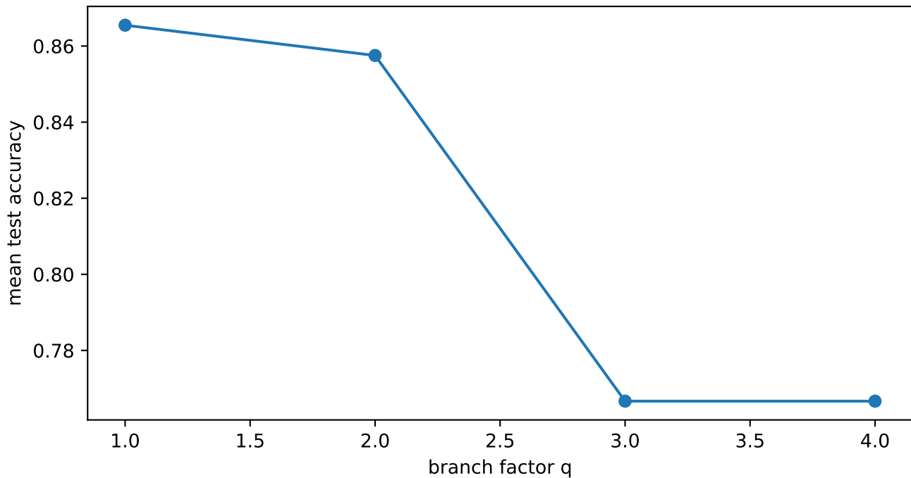
Nested primary accuracy
