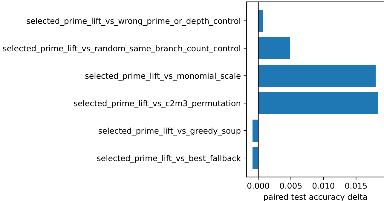
Selector regret / paired deltas
