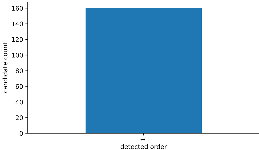
Torsion candidate orders
