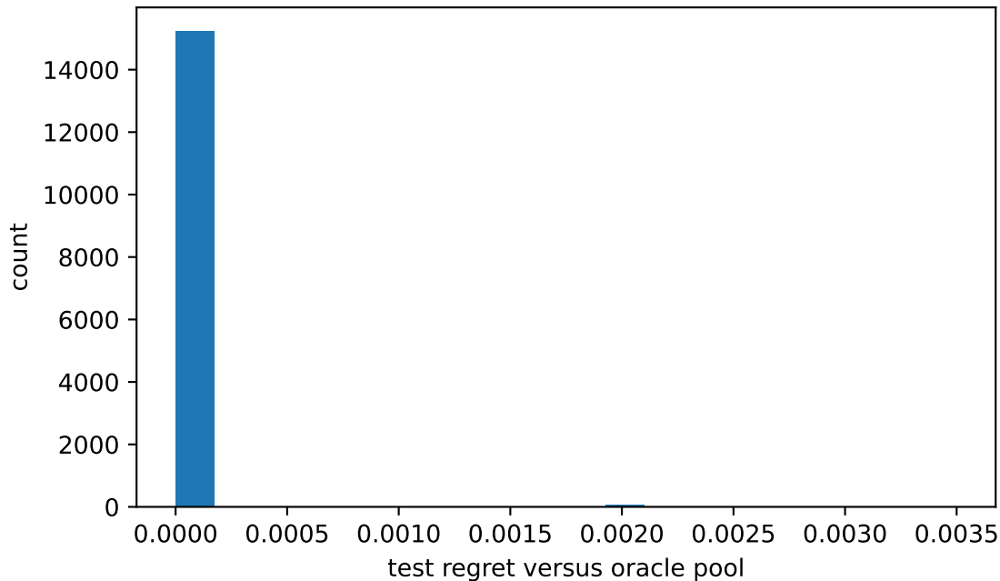
Torsion-safe selector regret
