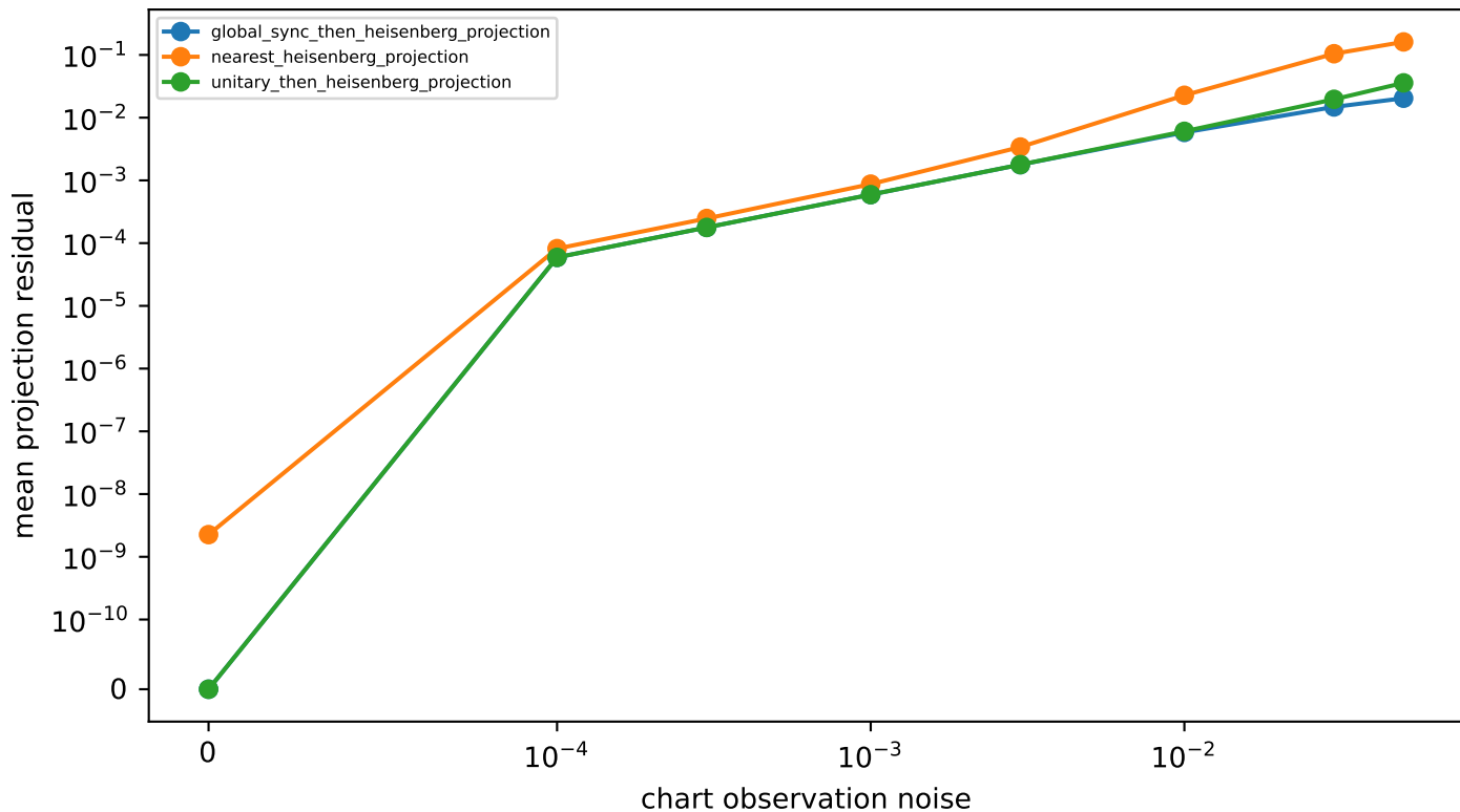
Nearest Heisenberg projection residual
