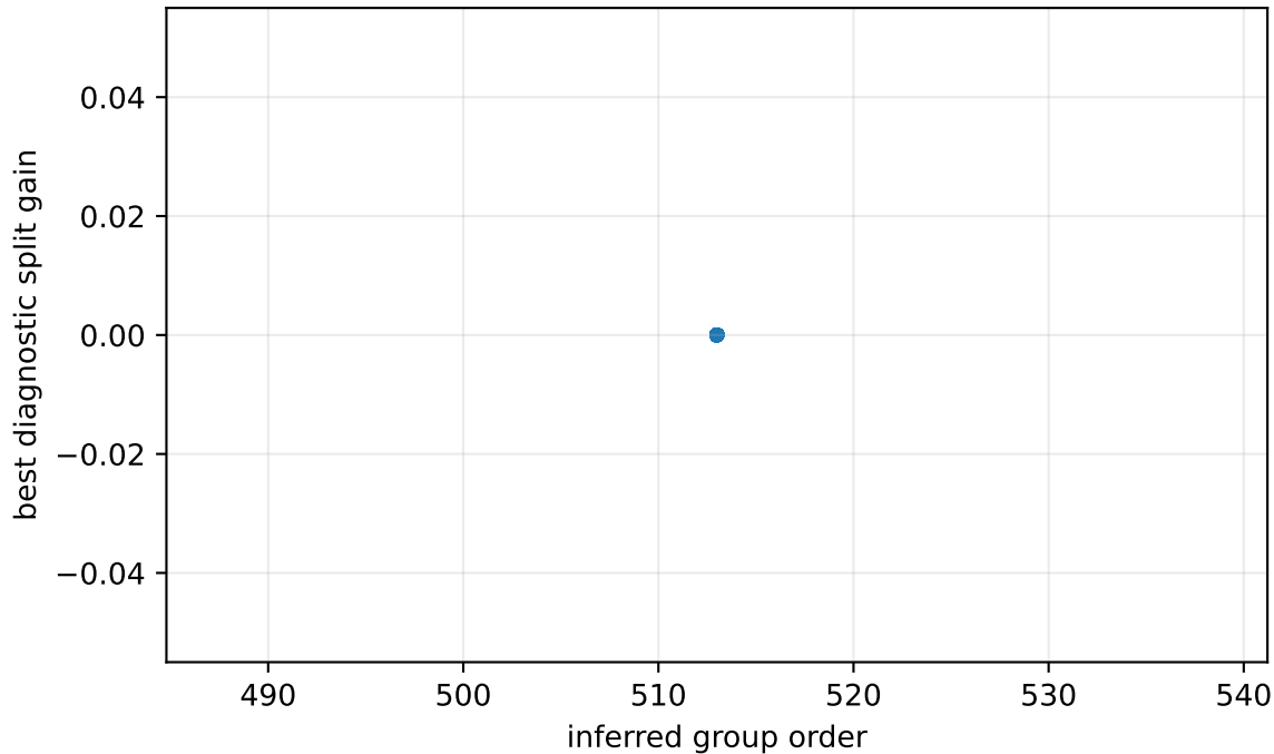
Group order versus split gain
