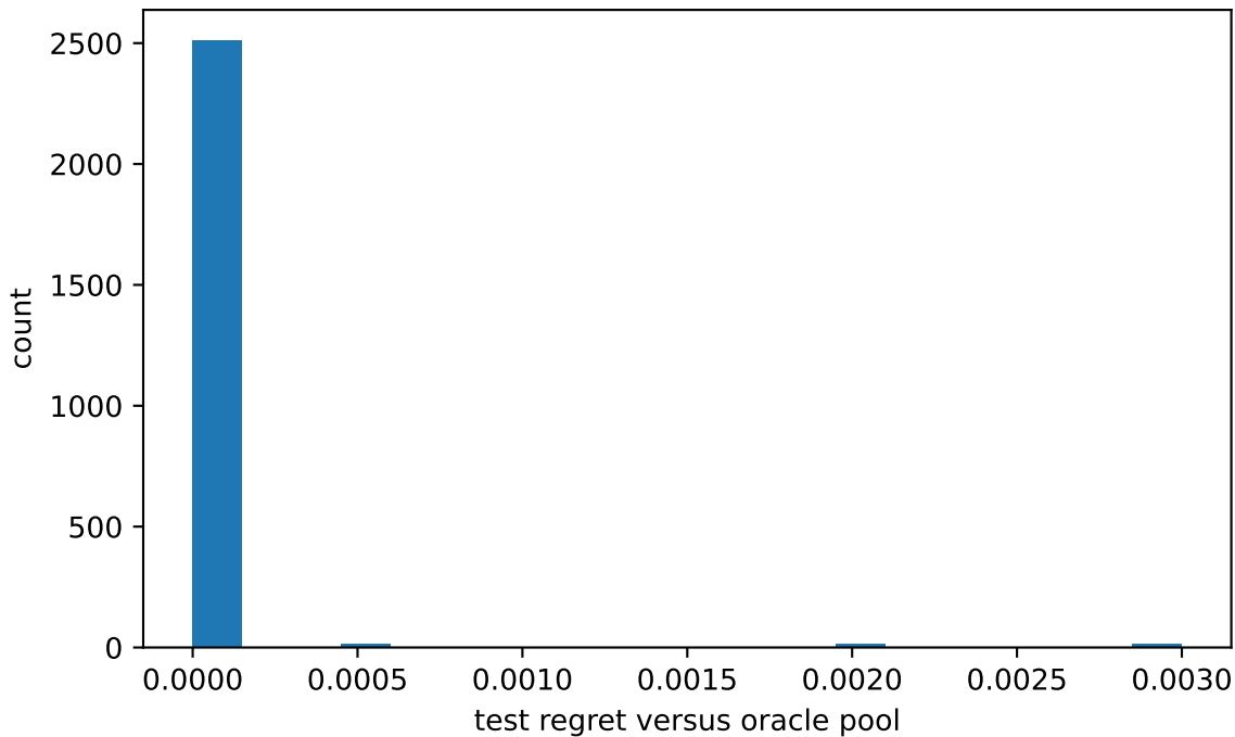
Nonabelian selector regret
