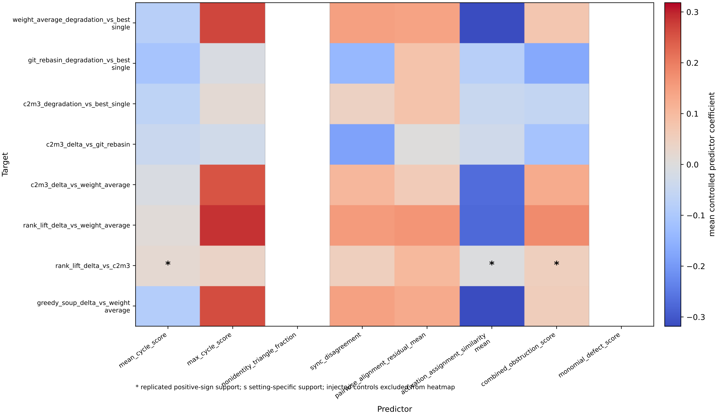
Observed predictor coefficients on full quality-gated fixed-setting data
