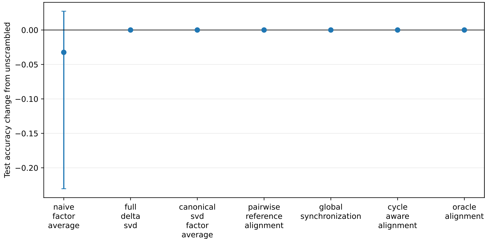
End-to-end stability across equivalent gauges
