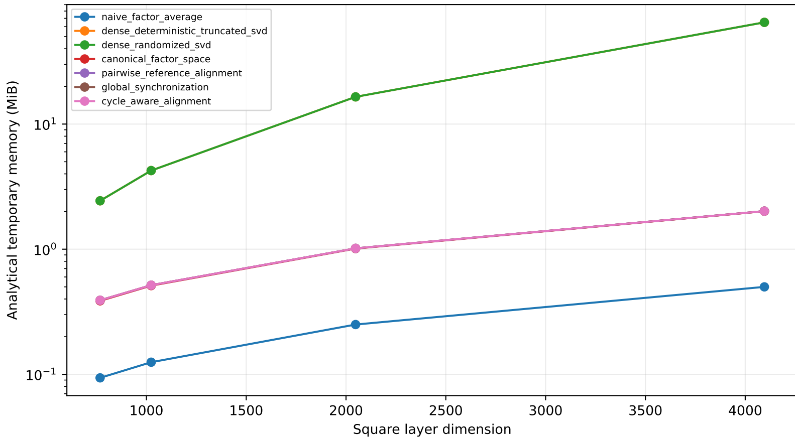
Low-rank-native versus dense temporary memory
