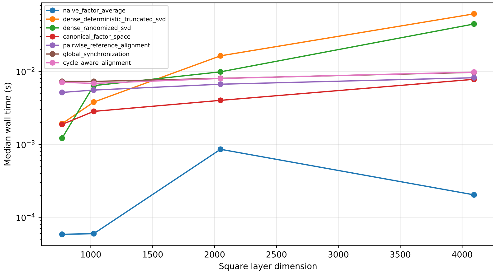
LoRA merge runtime, rank 8, 8 adapters
