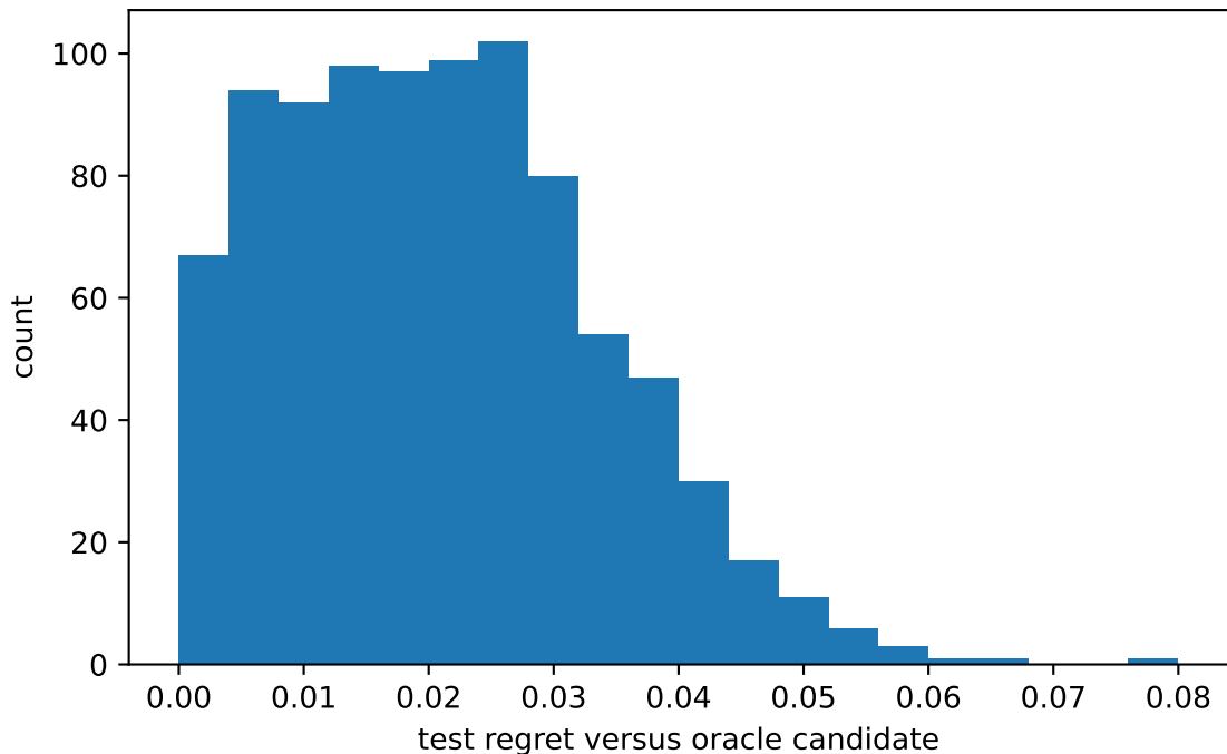
Controlled selector regret
