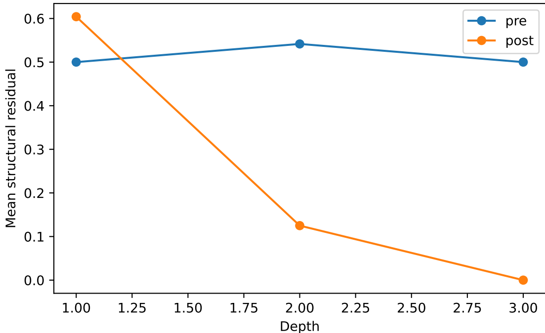
Residual by quotient-chain depth
