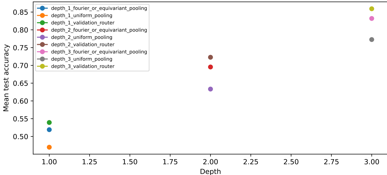
Controlled sequential quotient accuracy by depth
