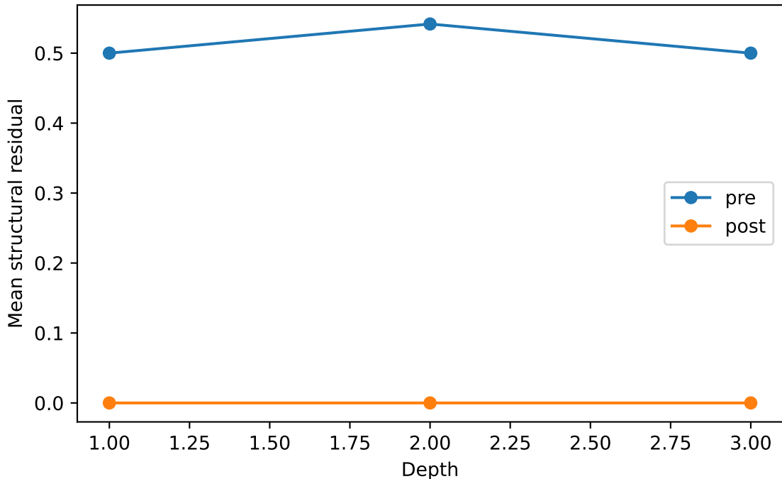
Residual by quotient-lift depth
