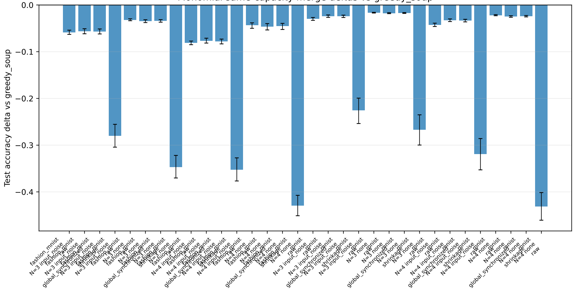
Monomial same-capacity merge deltas vs greedy_soup
