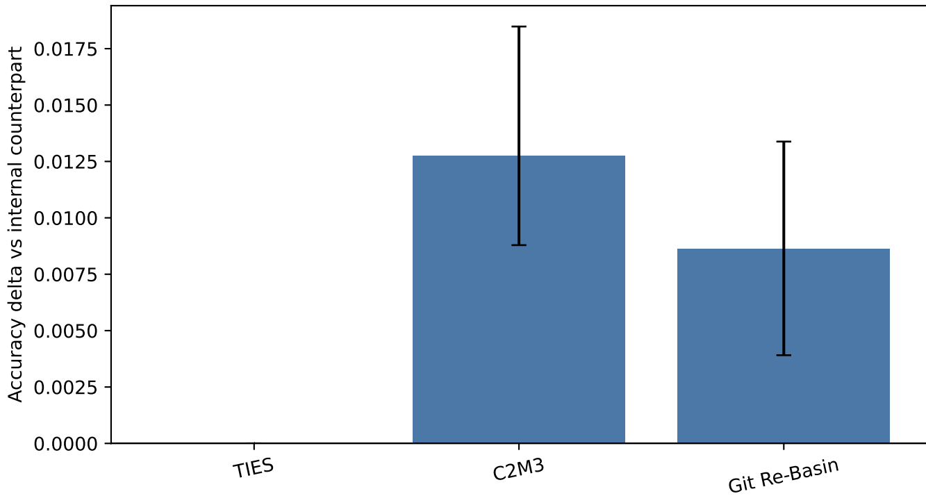
Adapter-assisted official-core comparisons
