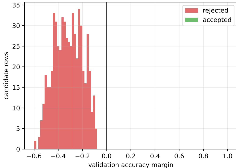
Decision boundary
