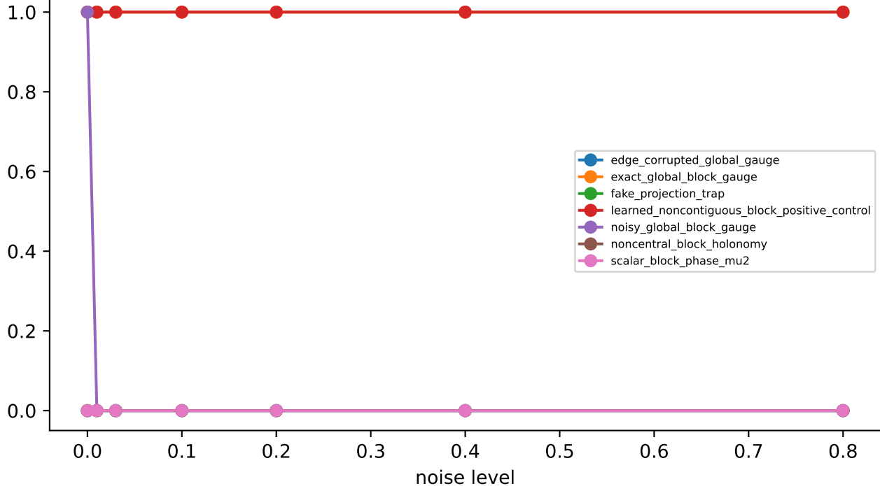
strict acceptance rate
