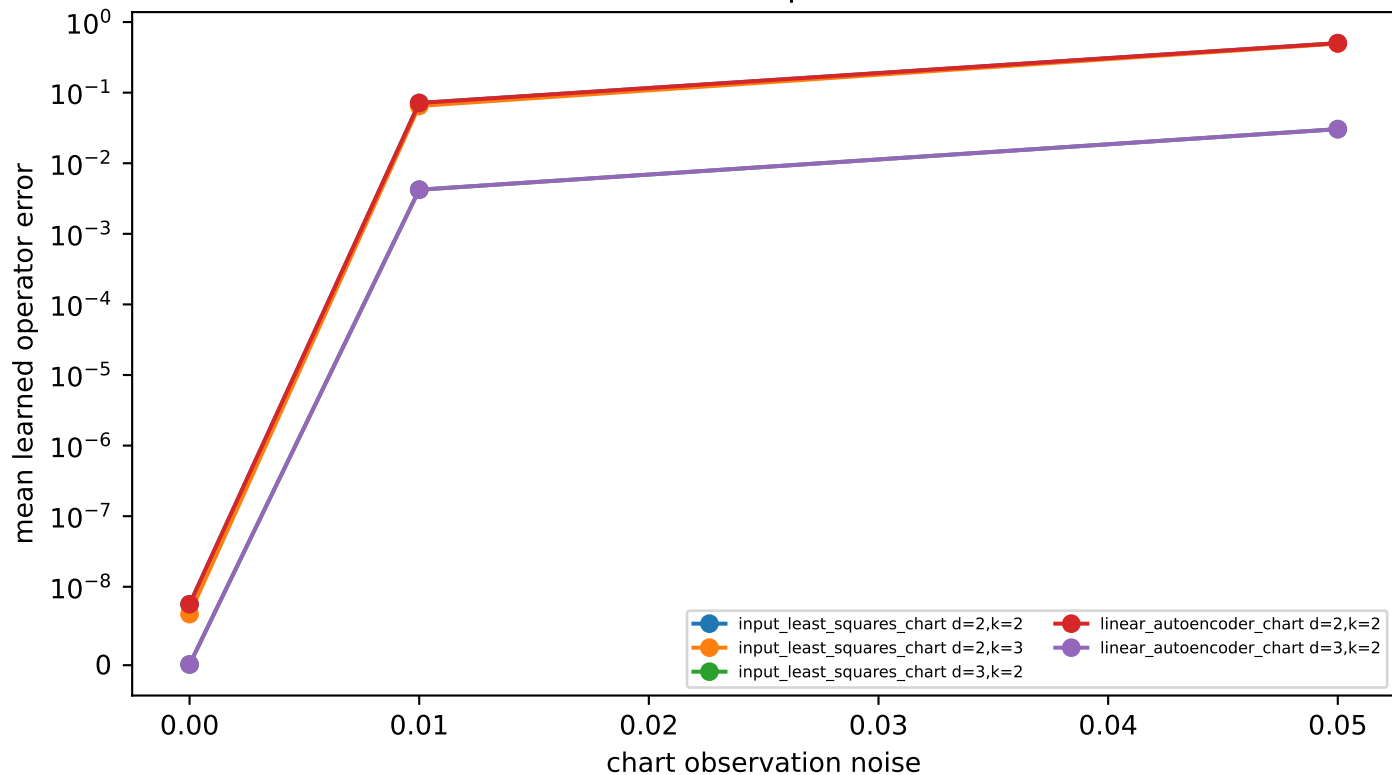
Learned chart operator error
