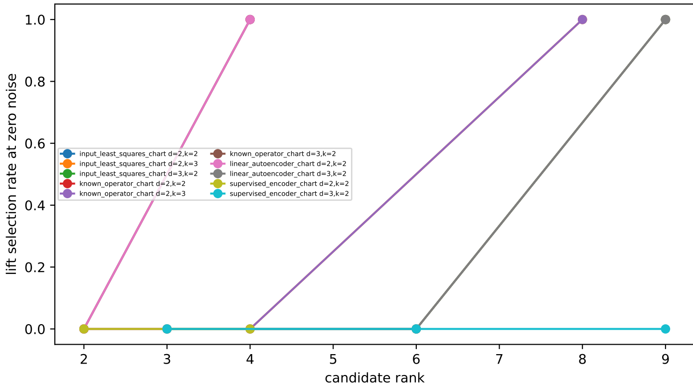
Learned chart rank threshold
