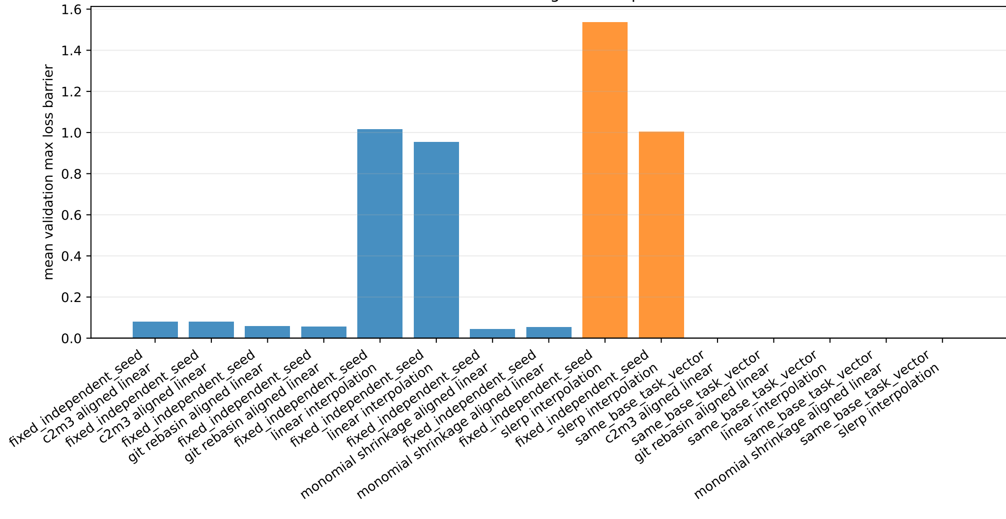
SLERP versus linear and aligned interpolation barriers
