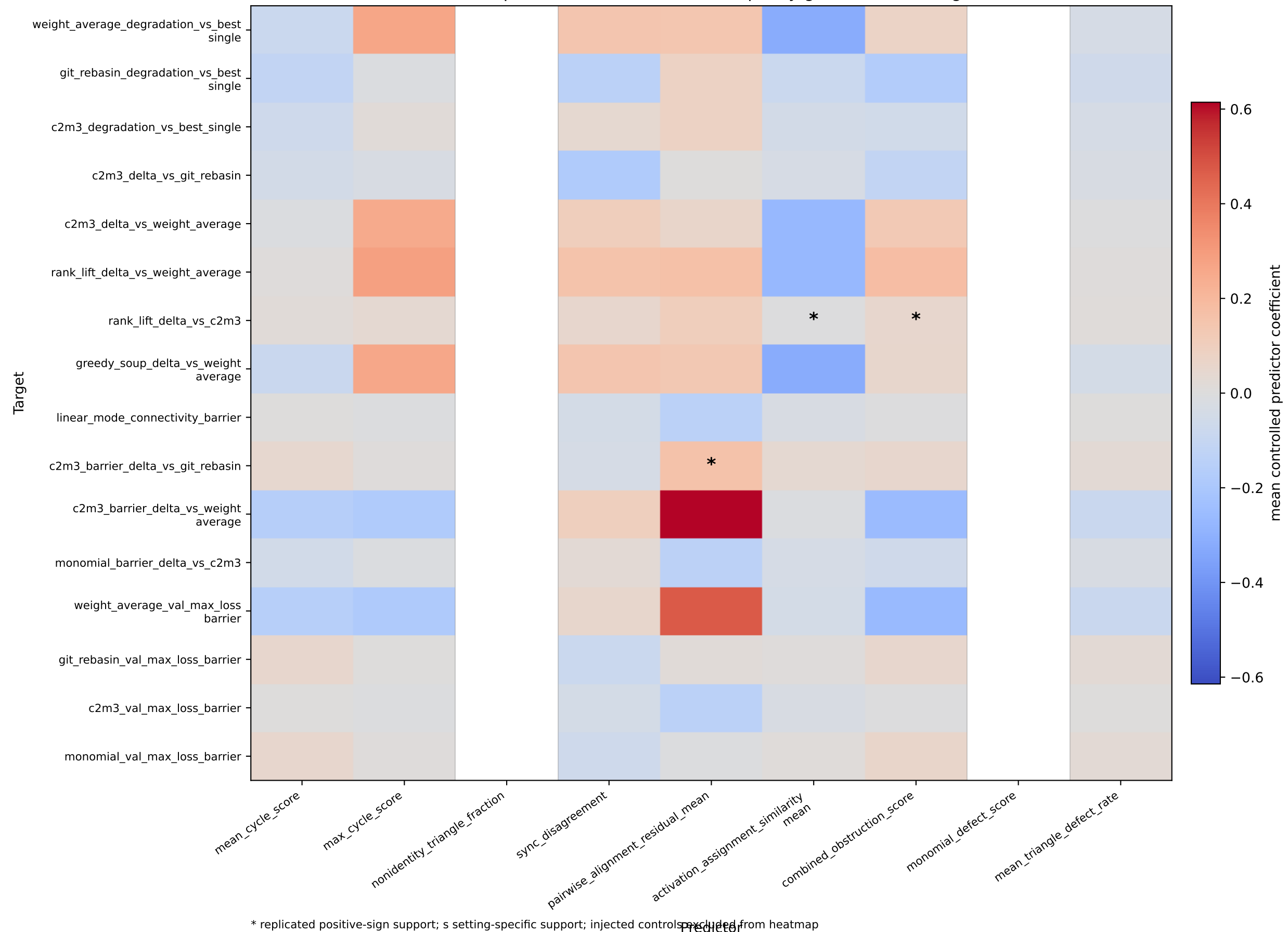
Observed predictor coefficients on full quality-gated fixed-setting data
