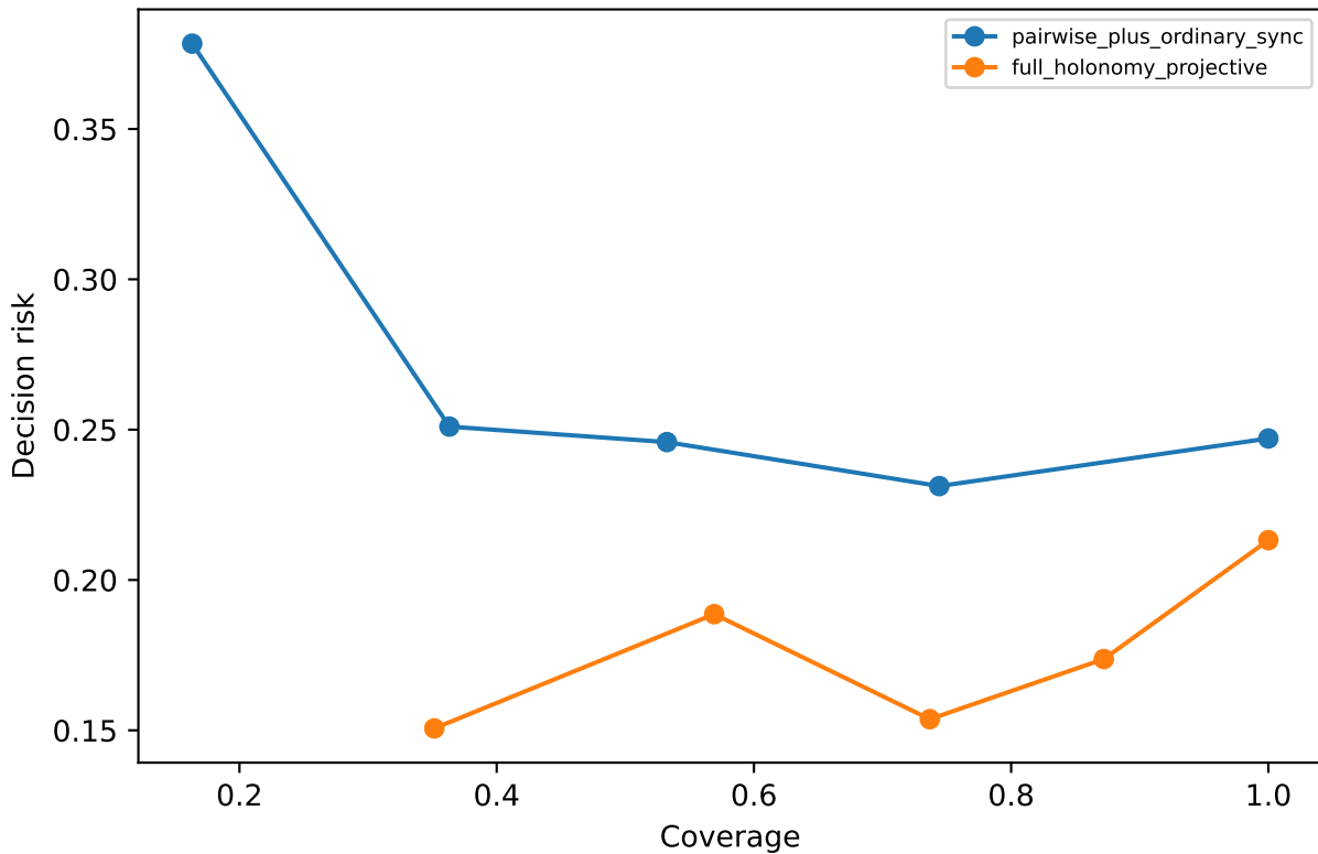
Merge/abstain coverage-risk
