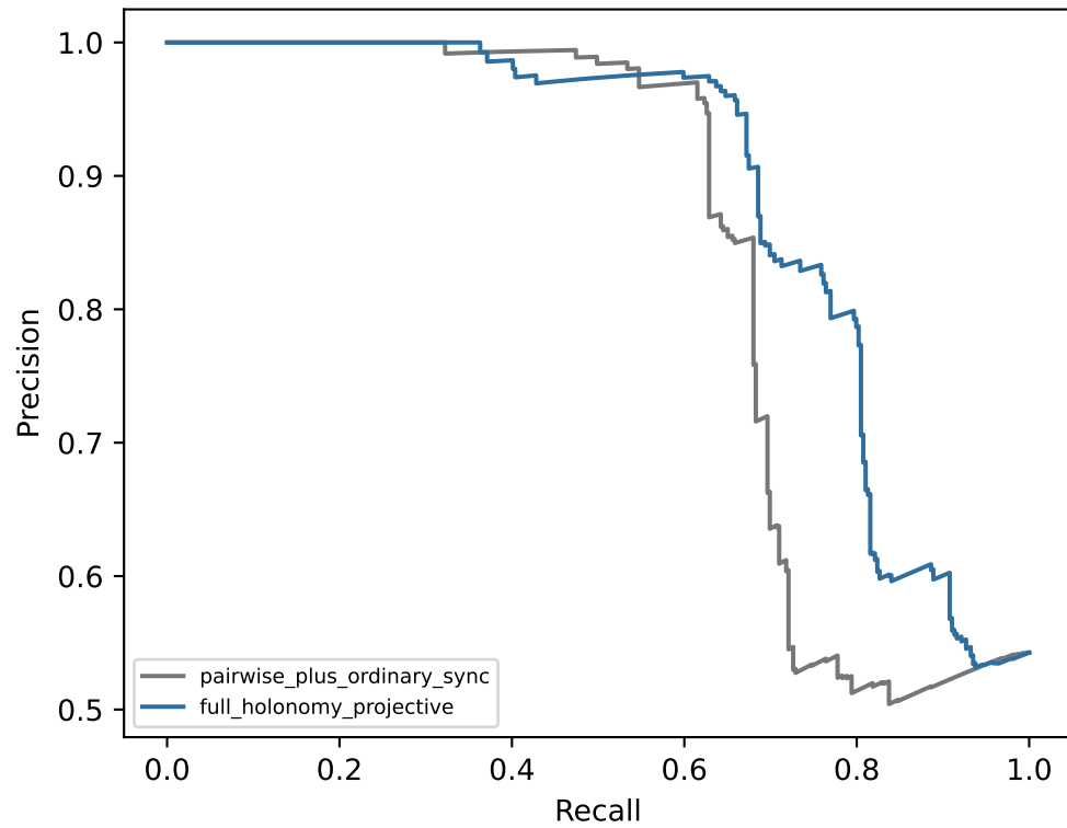
Double-held-out precision-recall
