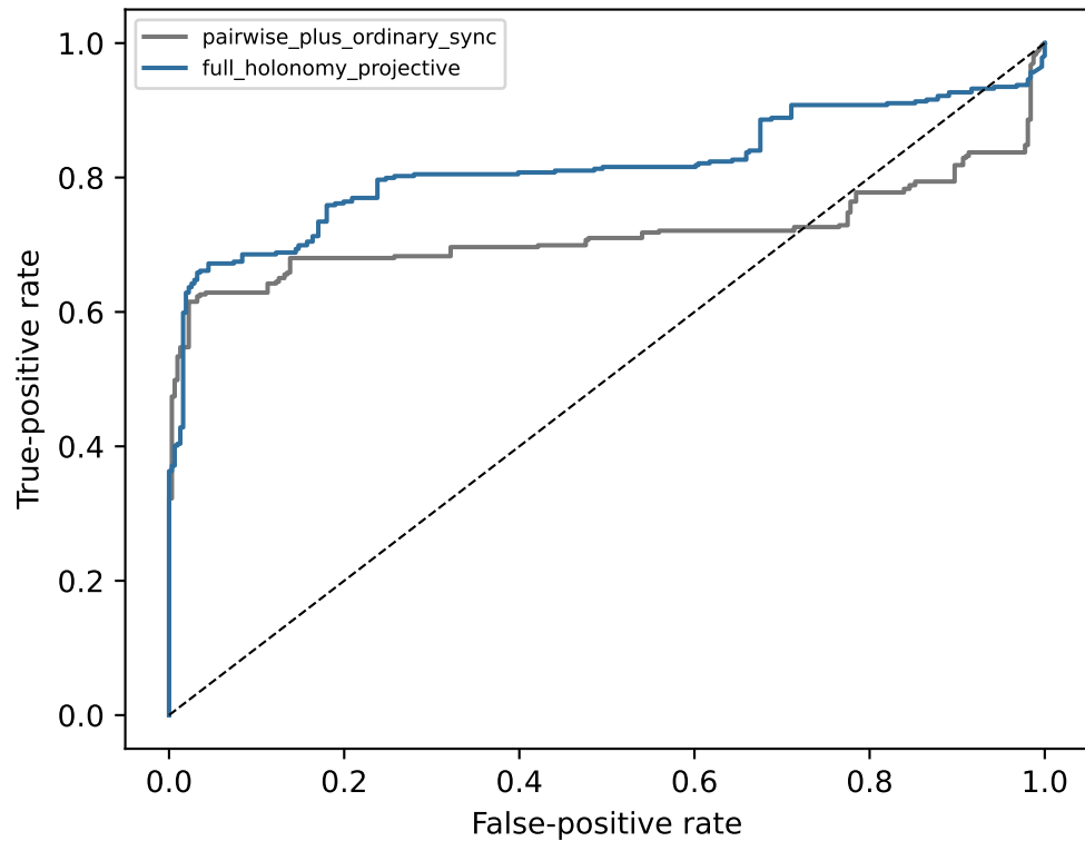
Double-held-out ROC
