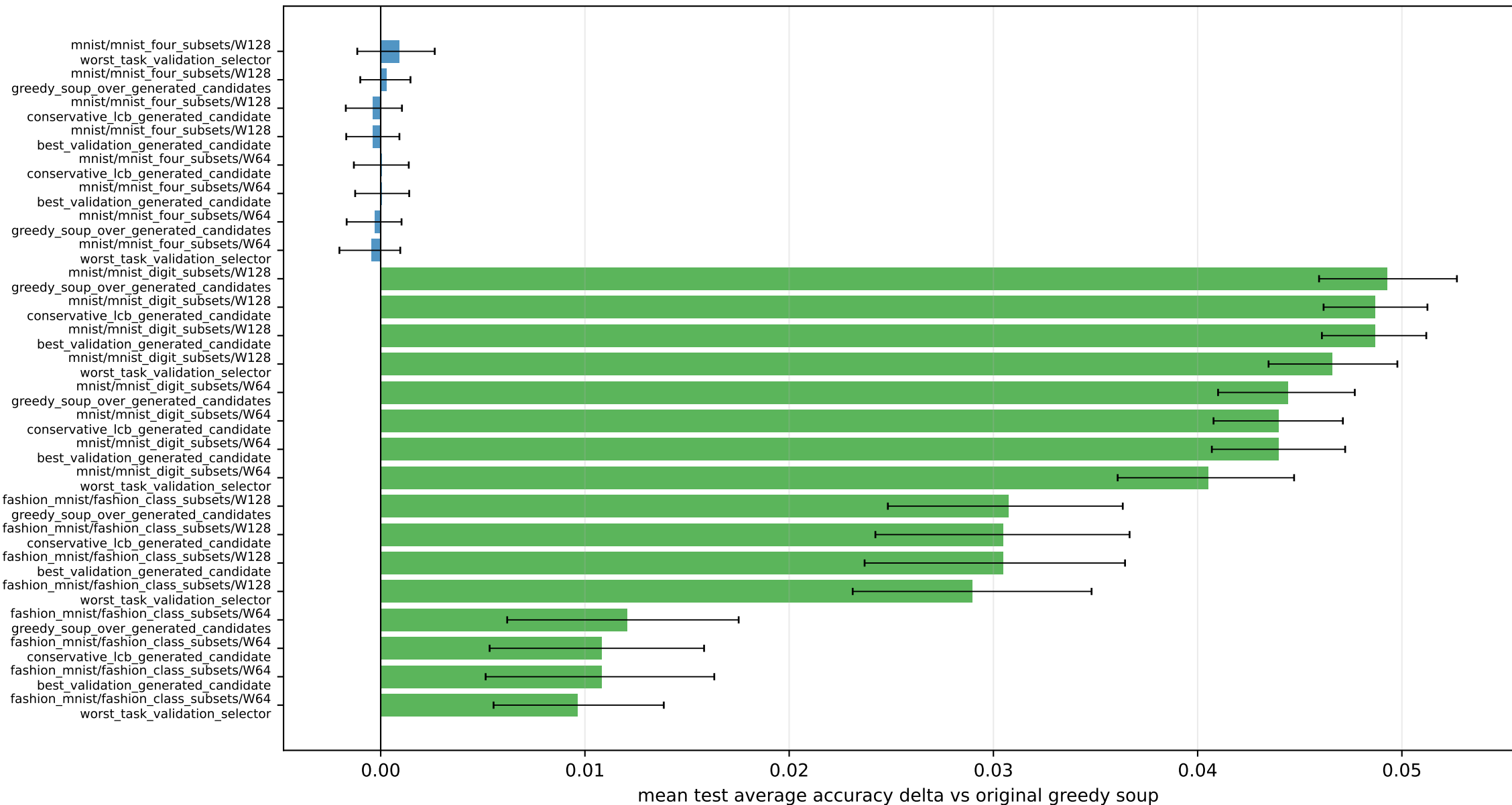
Descent envelope selectors over generated same-base candidates
