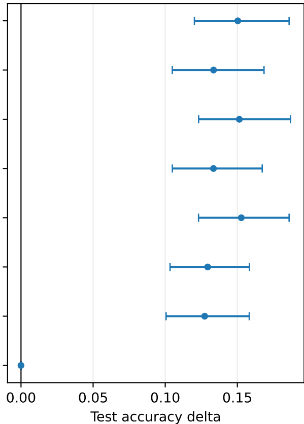
Delta vs weight average
