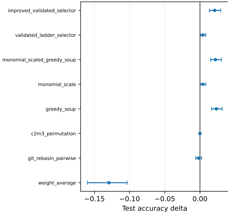
Delta vs internal C2M3
