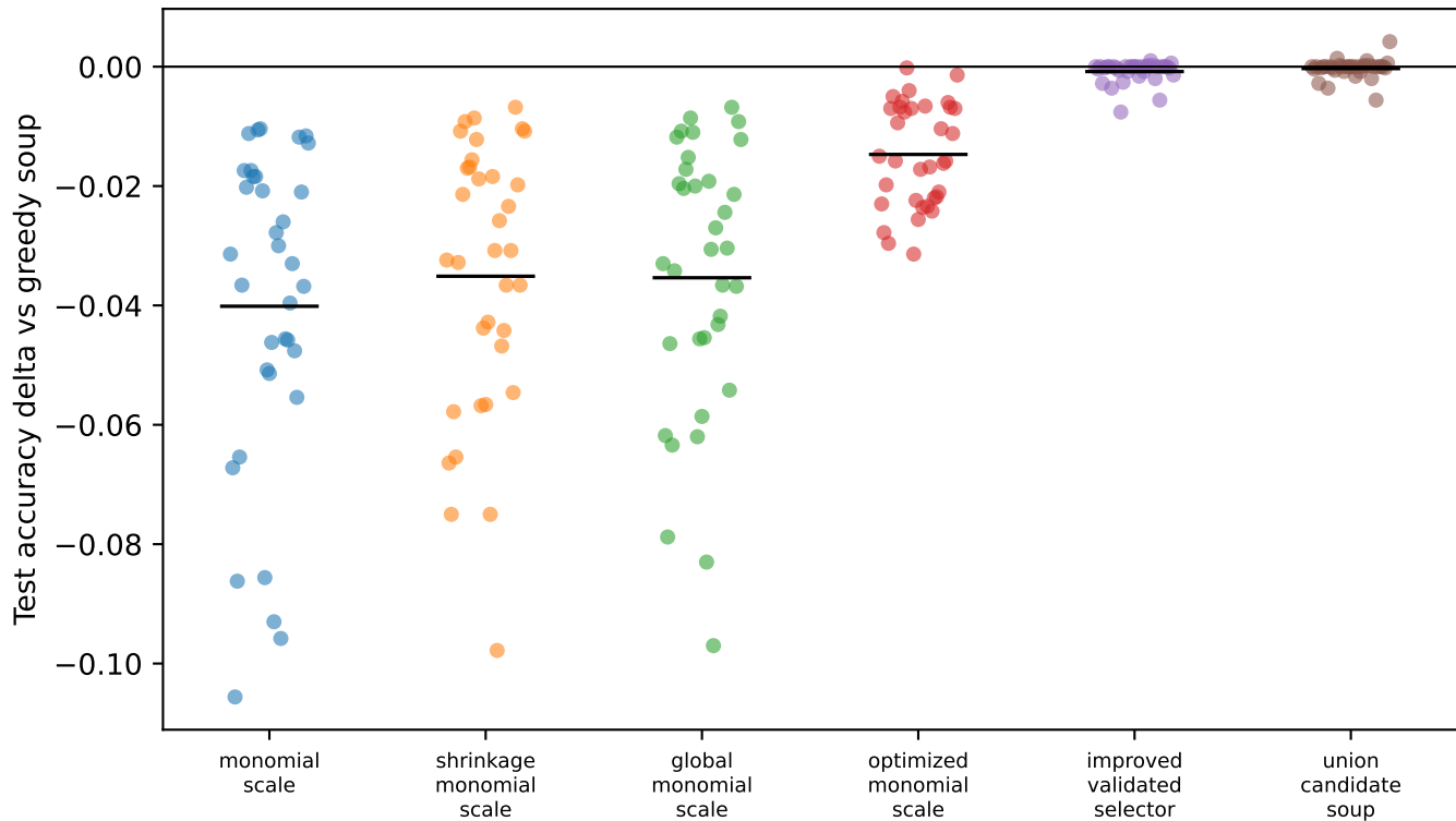
Fashion-MNIST Delta vs Greedy Soup
