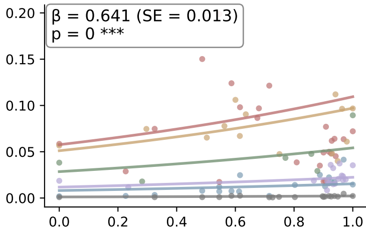
ParakeetV3
