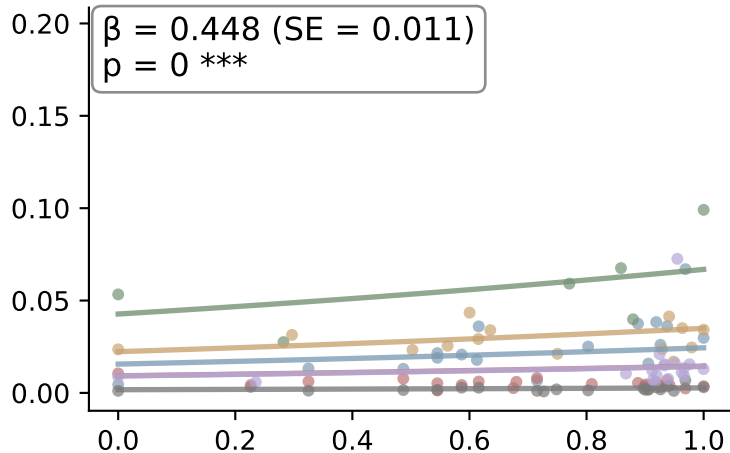
ParakeetV3
