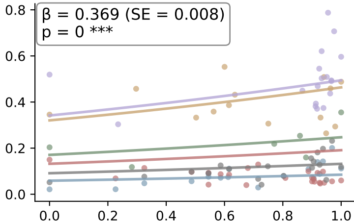
ParakeetV3
