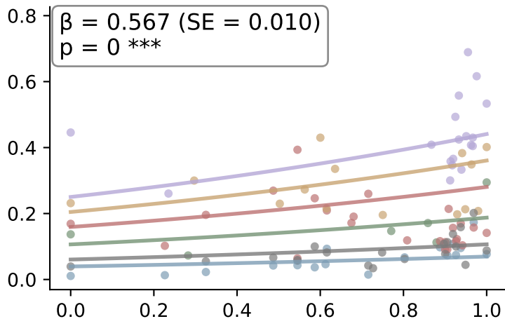
ParakeetV3
