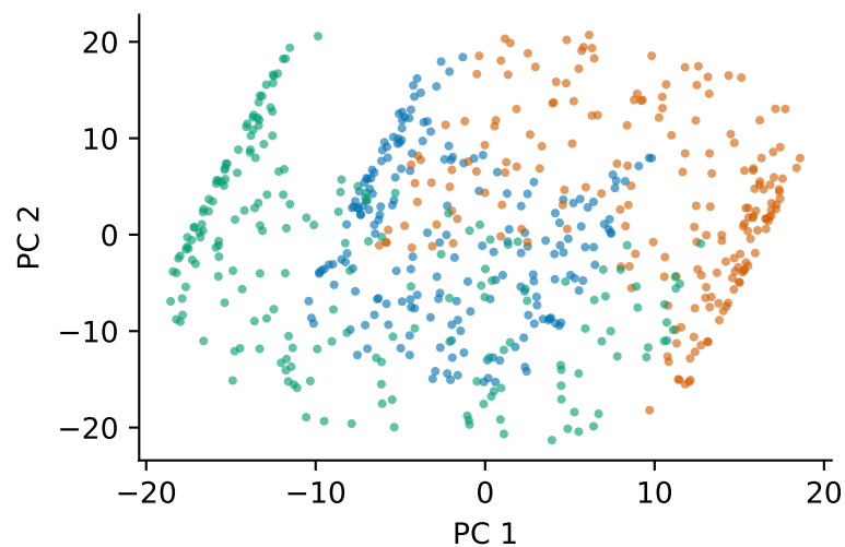
Swiss roll, d = 256
