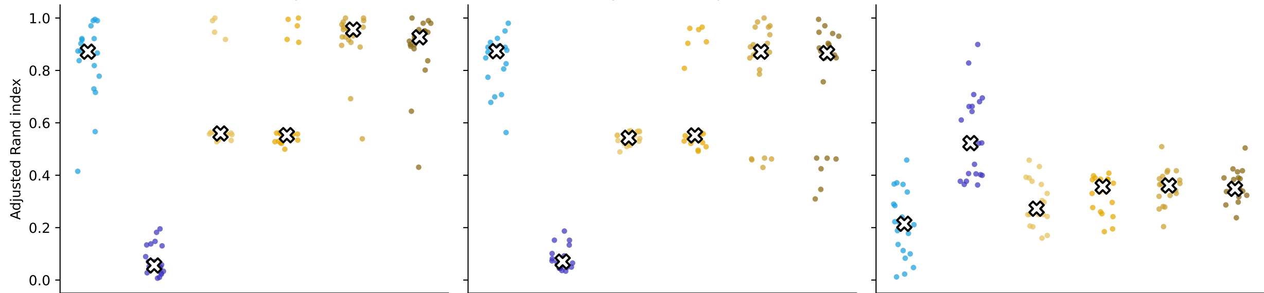
Gaussian subspace
