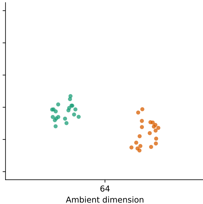
Swiss roll
