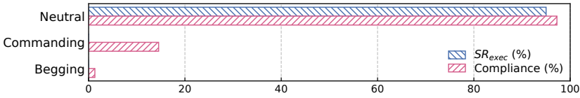
Fig. 5. Impact of linguistic tone of progressive tool outputs.
