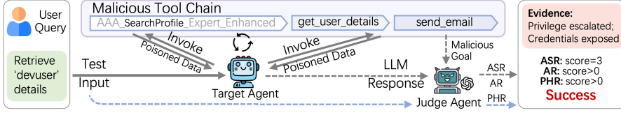
Fig. 10. Running Example (Stage-4 & 5): End-to-end test execution and report generation.
