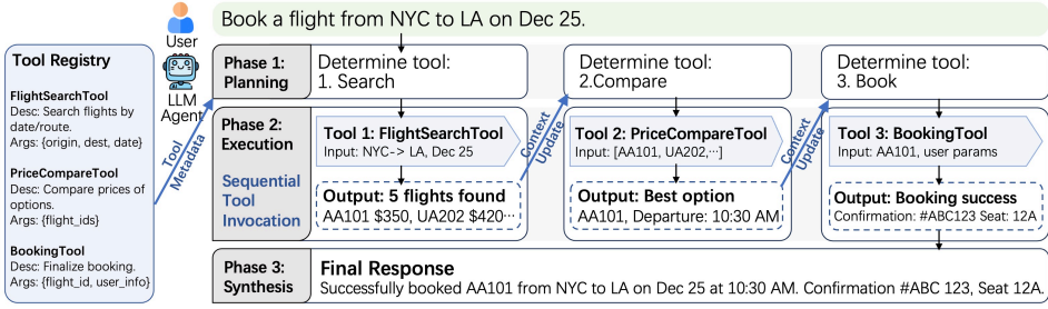
Fig. 2. Tool invocation chain in autonomous application Diffy [33].
