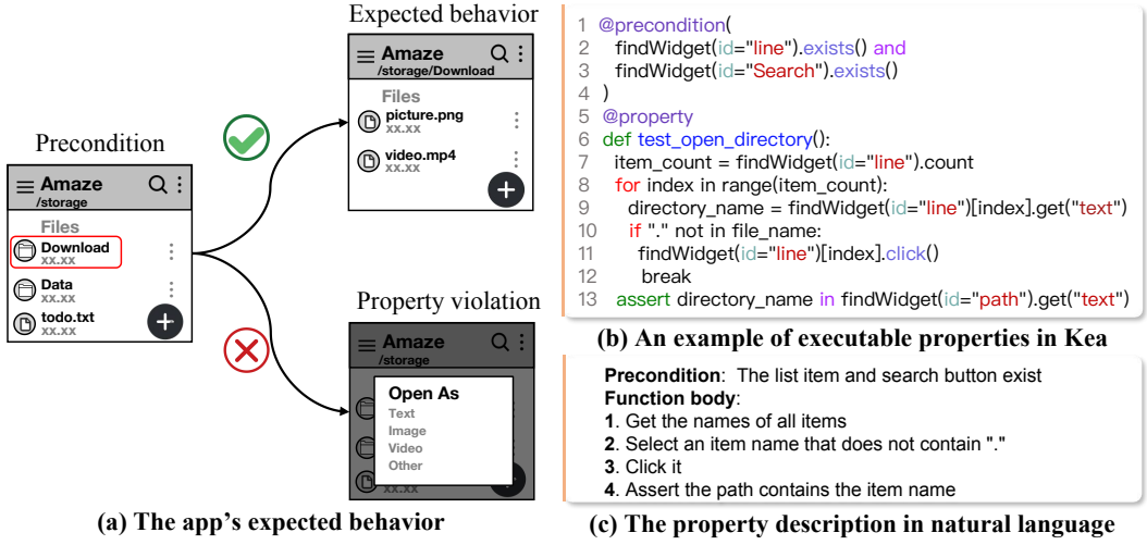
Fig. 1. An example of the property in app Amaze.
