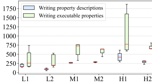
Fig. 4. Time consumption of participants in writing property descriptions and executable properties. The x-axis represents different properties, and the y-axis represents the time spent (in seconds).
