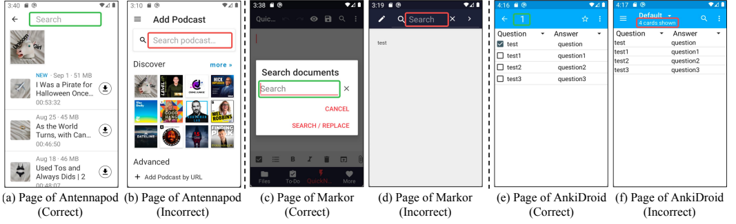
Fig. 3. Examples of failure cases. The green boxes annotate the correct widgets and red boxes annotate the incorrect widgets.
