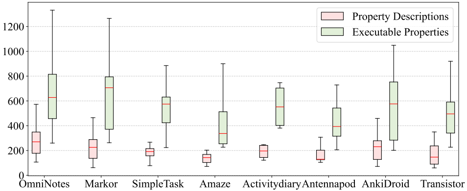
Fig. 5. Comparison of the complexity (measured in character count) between natural language property descriptions and their corresponding executable properties across eight Android apps.
