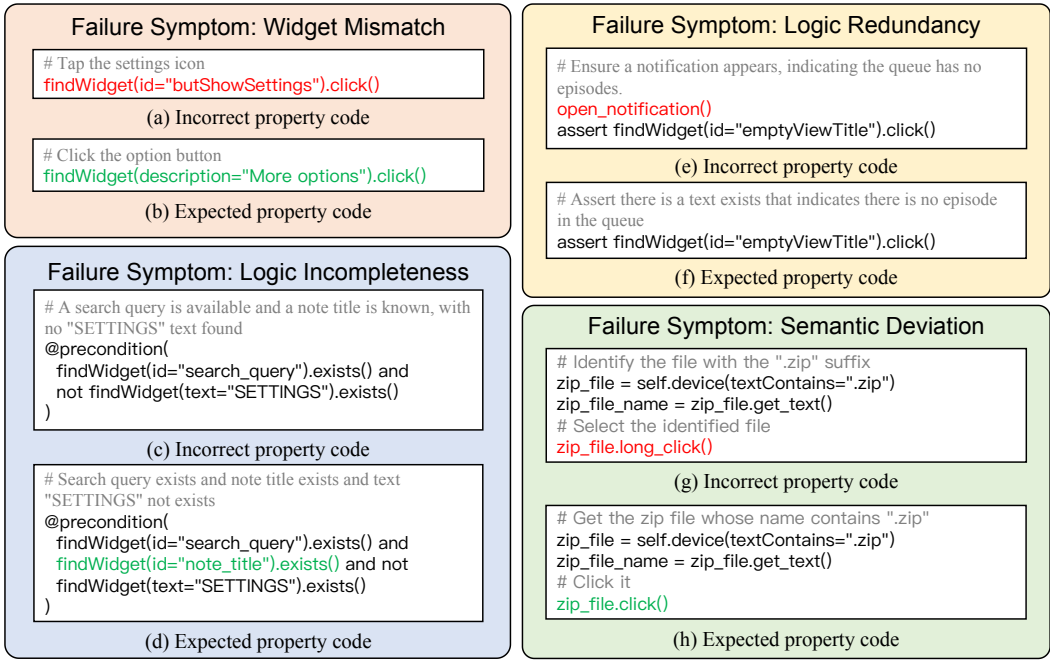
Fig. 8. Illustrative examples of failure symptoms. Incorrect and correct implementations are marked in red and green, respectively, with property descriptions in gray (code snippets are simplified for clarity).
