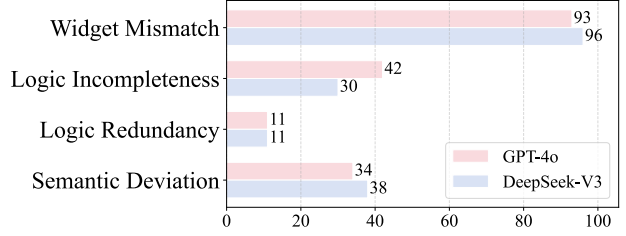
Fig. 7. Failure symptom distribution.
