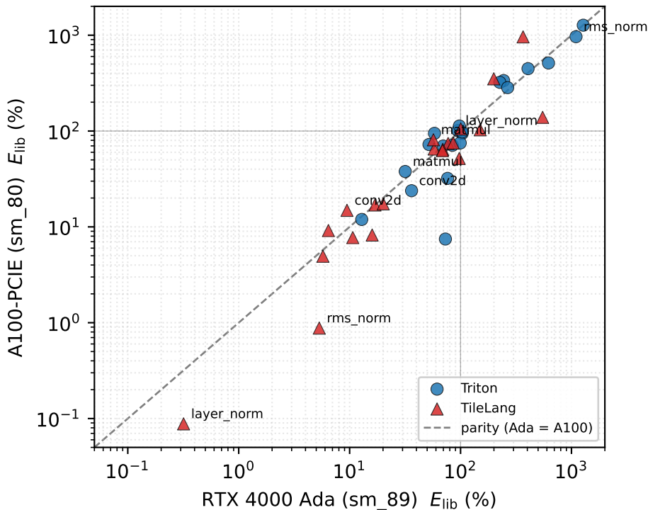
Per-kernel DSL efficiency tracks across architectures
