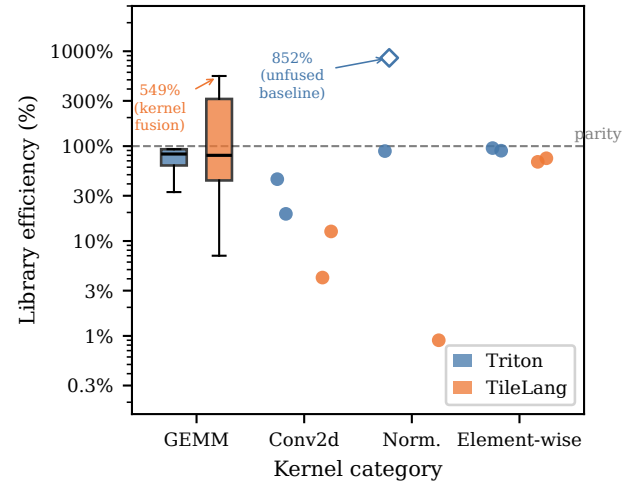
Figure 1: Library efficiency (%) of Triton and TileLang kernels relative to cuBLAS/cuDNN on the NVIDIA A100-SXM4-40GB, grouped by kernel category (log scale). GEMM shows boxes (IQR; whiskers 1.5\times IQR); all other categories show individual kernel measurements as dots ( n = 2 per cell). Dashed line marks parity (100%). The hollow diamond at 851.8% (Triton, Norm.) marks Triton rms_norm : the PyTorch eager baseline does not fuse its normalization passes, making this an unfair comparison rather than a genuine DSL win; see section 5.3. The boxplot flier at 548.6% (TileLang, GEMM) marks fused linear+activation, a valid DSL advantage through kernel fusion; see section 5.3. Attention excluded; see section 5.3.
