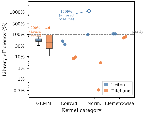
Figure 1: Library efficiency (%) of Triton and TileLang kernels relative to cuBLAS/cuDNN, grouped by kernel category (log scale). GEMM shows boxes (IQR; whiskers 1.5 \times IQR); all other categories show individual kernel measurements as dots ( n = 2 per cell). Dashed line marks parity (100%). The hollow diamond at 1099% (Triton, Norm.) marks Triton rms.norm: the PyTorch eager baseline does not fuse its normalization passes, making this an unfair comparison rather than a genuine DSL win; see section 5.1. The boxplot flier at 200% (TileLang, GEMM) marks fused linear+activation, a valid DSL advantage through kernel fusion; see section 5.1. Attention excluded; see section 5.1.
