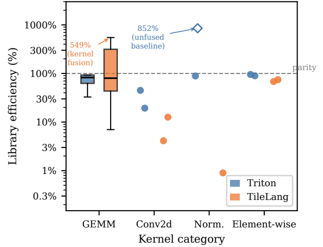
Fig. 1. Library efficiency (%) of Triton and TileLang kernels relative to cuBLAS/cuDNN on the NVIDIA A100-SXM4-40GB, grouped by kernel category (log scale). GEMM shows boxes (IQR; whiskers 1.5\times IQR); all other categories show individual kernel measurements as dots ( n = 2 per cell). Dashed line marks parity (100%). The hollow diamond at 851.8% (Triton, Norm.) marks Triton rms_norm : the PyTorch eager baseline does not fuse its normalization passes, making this an unfair comparison rather than a genuine DSL win; see table III. The boxplot flier at 548.6% (TileLang, GEMM) marks fused linear+activation , a valid DSL advantage through kernel fusion; see section V-C. Attention excluded; see section V-C.
