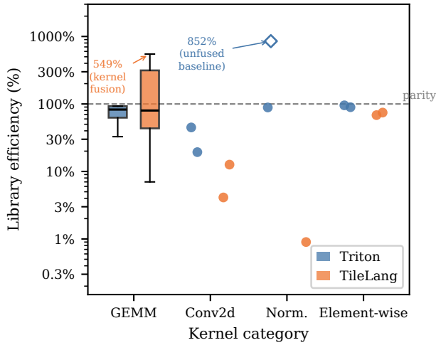
Figure 1: Library efficiency (%) of Triton and TileLang kernels relative to cuBLAS/cuDNN on the NVIDIA A100-SXM4-40GB, grouped by kernel category (log scale). GEMM shows boxes (IQR; whiskers 1.5 \times IQR); all other categories show individual kernel measurements as dots ( n = 2 per cell). Dashed line marks parity (100%). The hollow diamond at 851.8% (Triton, Norm.) marks Triton rms.norm: the PyTorch eager baseline does not fuse its normalization passes, making this an unfair comparison rather than a genuine DSL win; see section 5.3. The boxplot flier at 548.6% (TileLang, GEMM) marks fused linear+activation, a valid DSL advantage through kernel fusion; see section 5.3. Attention excluded; see section 5.3.
